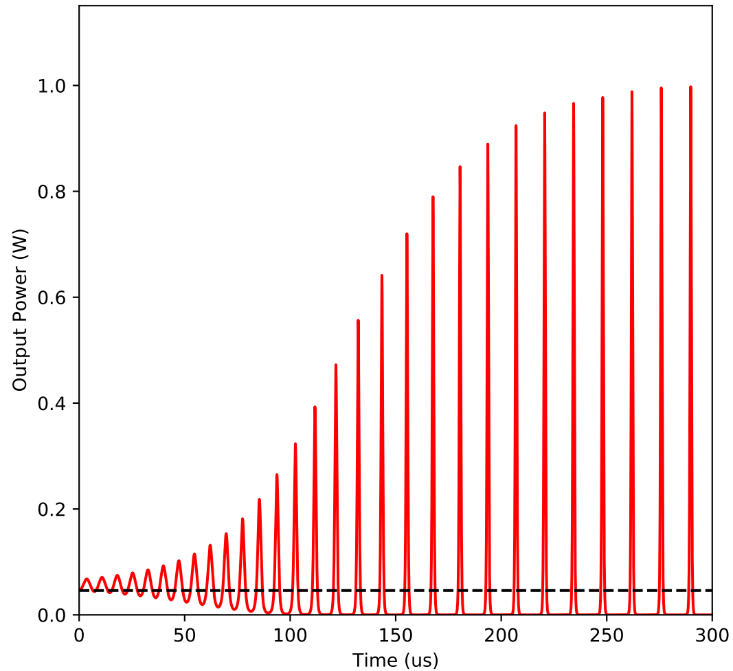
Q-Switching
